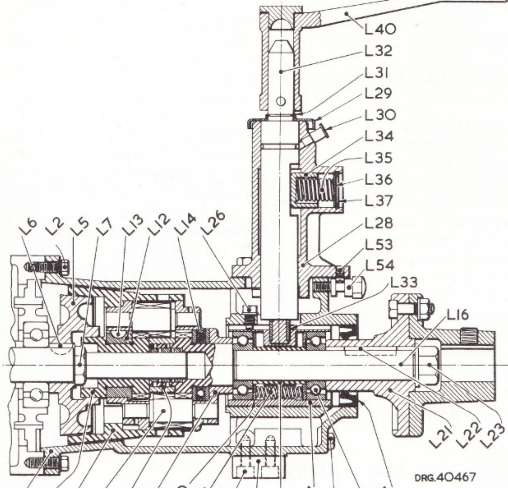
Reverse Gearbox
